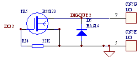
Digital Output Circuit
