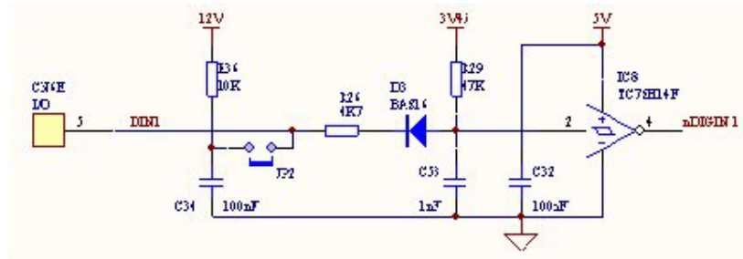
Digital Input Circuit
